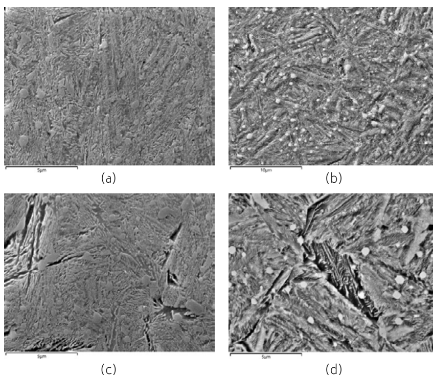
Fig.8 - SE-SEM micrographs of the EN 100Cr6 steel austenitized at 880 °C for 150 min + salt quenching at 240 °C: (a) 60 min holding time in the upper surface of the ring, (b) 300 min holding time in the upper surface of the ring, (c) 60 min holding time in the central region of the ring, (d) 300 min holding time in the central region of the ring
