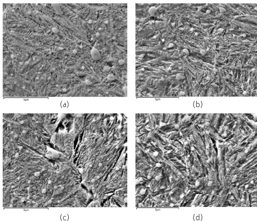
Fig.9 - SE-SEM micrographs of the EN 100Cr6 steel austenitized at 880 °C for 150 min + salt quenching at 220 °C: (a) 60 min holding time in the upper surface of the ring, (b) 300 min holding time in the upper surface of the ring, (c) 60 min holding time in the central region of the ring, (d) 300 min holding time in the central region of the ring
