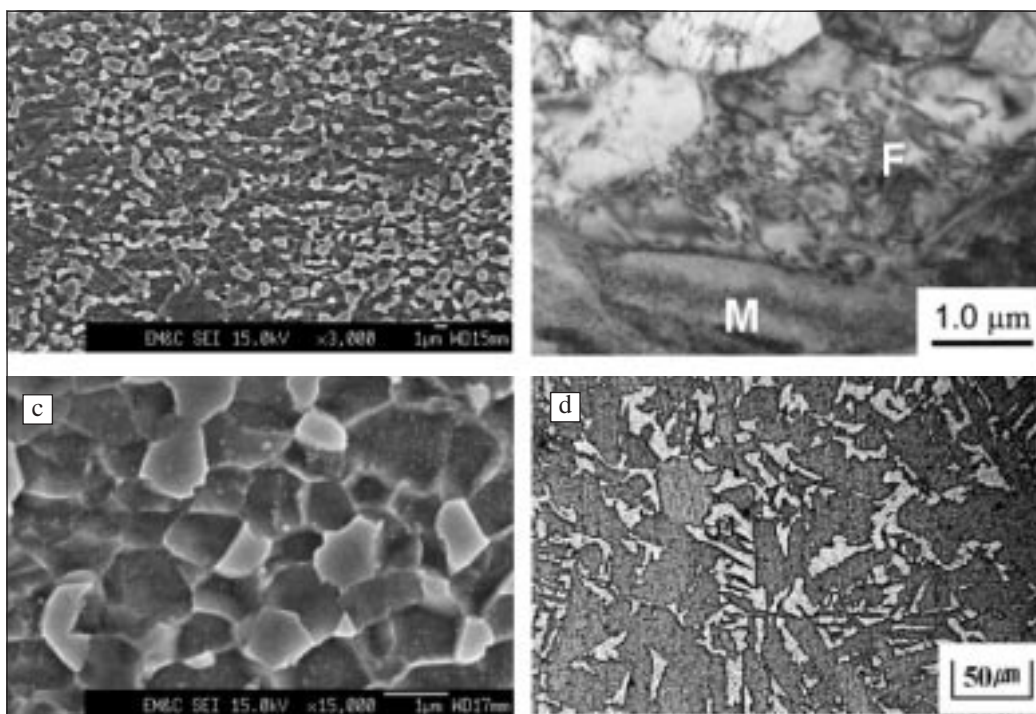
Fig. 7 – (a) SEM micrograph of the present dual phase steel, (b) TEM micrograph of the present dual phase steel, (c) SEM micrograph of the present dual phase steel with higher magnification, (d) Optical micrograph of the coarse dual phase steel (the white patches are martensite).
