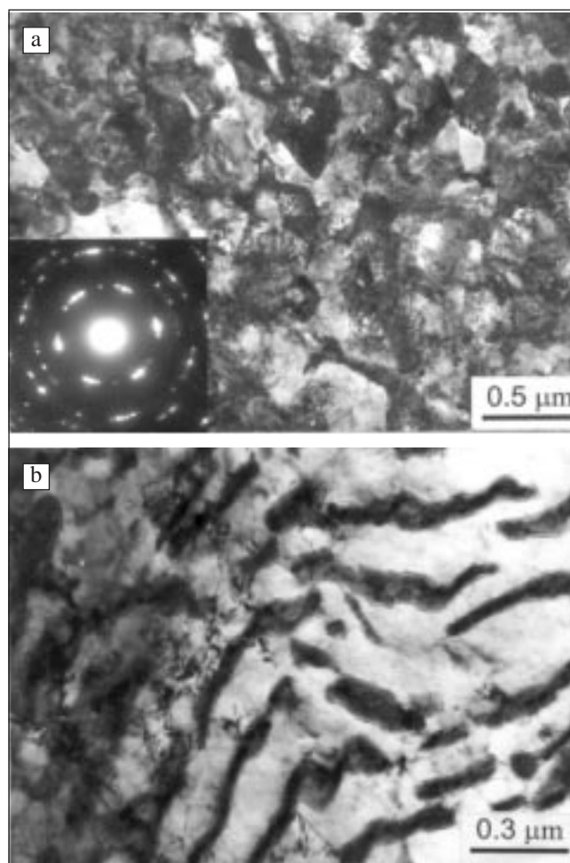
Fig. 1 – TEM micrographs of (a) ferrite and (b) pearlite of the present steel after ECAP.
