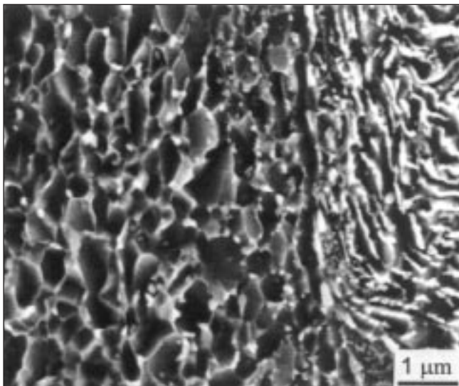
Fig. 2 – SEM micrograph showing the precipitation of nanosized cementite particles at UFG ferrite grain boundaries in the vicinity of pearlite colony in the present steel after ECAP followed by 873 K °φ 1 hr annealing.
