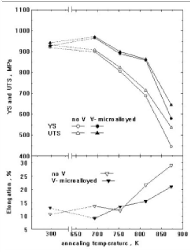
Fig. 6 – Comparison of the tensile properties between UFG steels with or without V as a function of annealing temperature (1 hr annealing).
