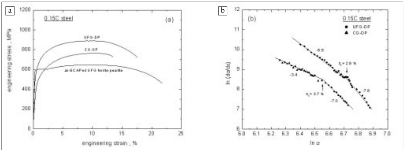
Fig. 8 – (a) Comparison of nominal stress-strain curves of the UFG dual phase steel, coarse grained dual phase steel, and UFG ferrite/pearlite phase steel, and (b) Comparison of the plot of the \ln (d\sigma/d\varepsilon) versus \ln \sigma between UFG-DP and CG-DP steels.
