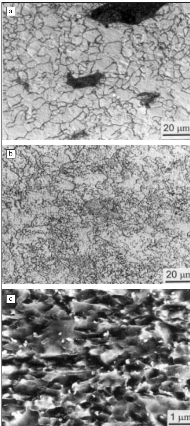
Fig. 4 – (a) Optical micrograph of the steel without V after ECAP and annealing at 873 K for 1 hr, (b) Optical and (c) SEM micrographs of the V microalloyed steel after ECAP and annealing at 873 K for 1 hr.
